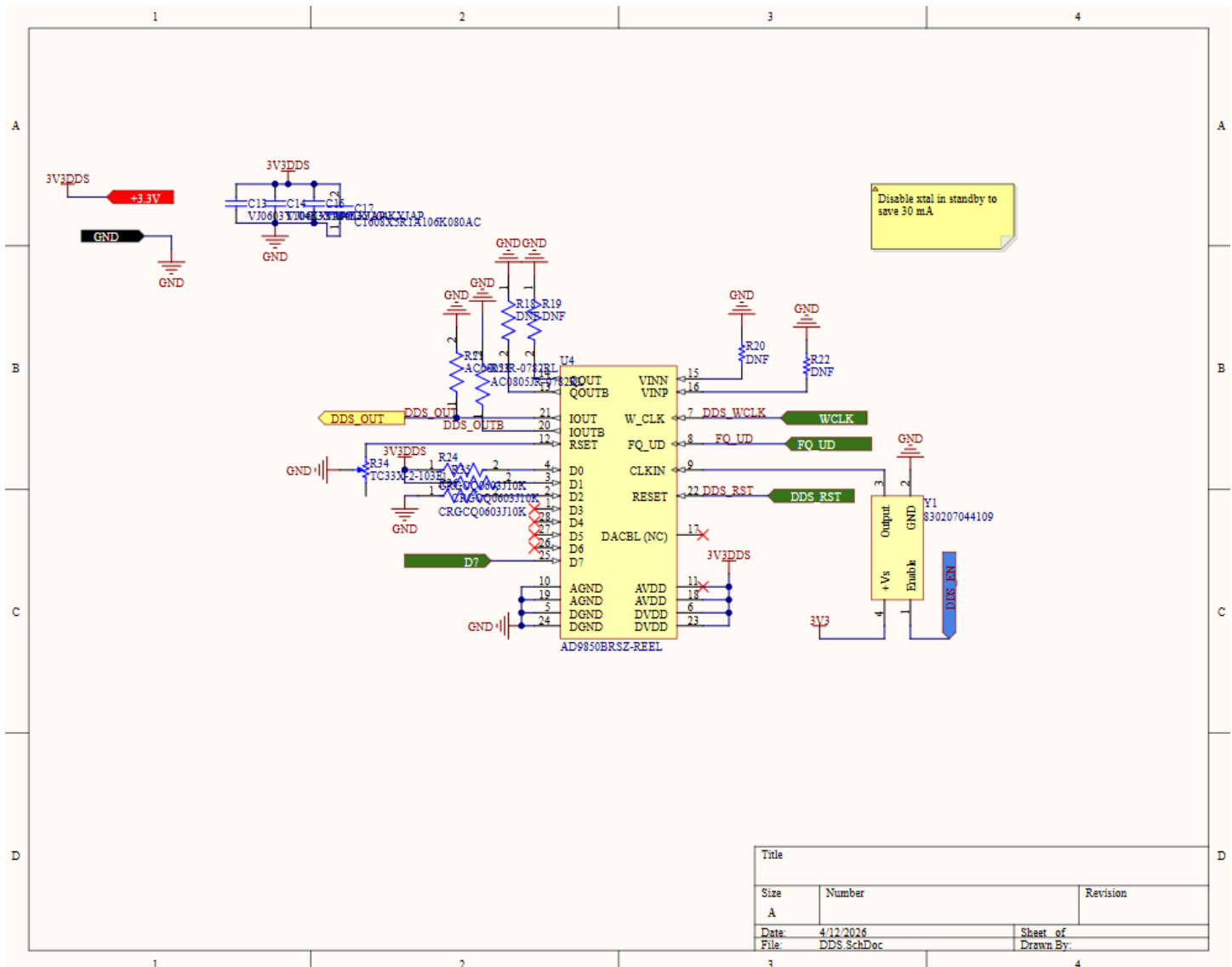
DDS sub-system schematic.
