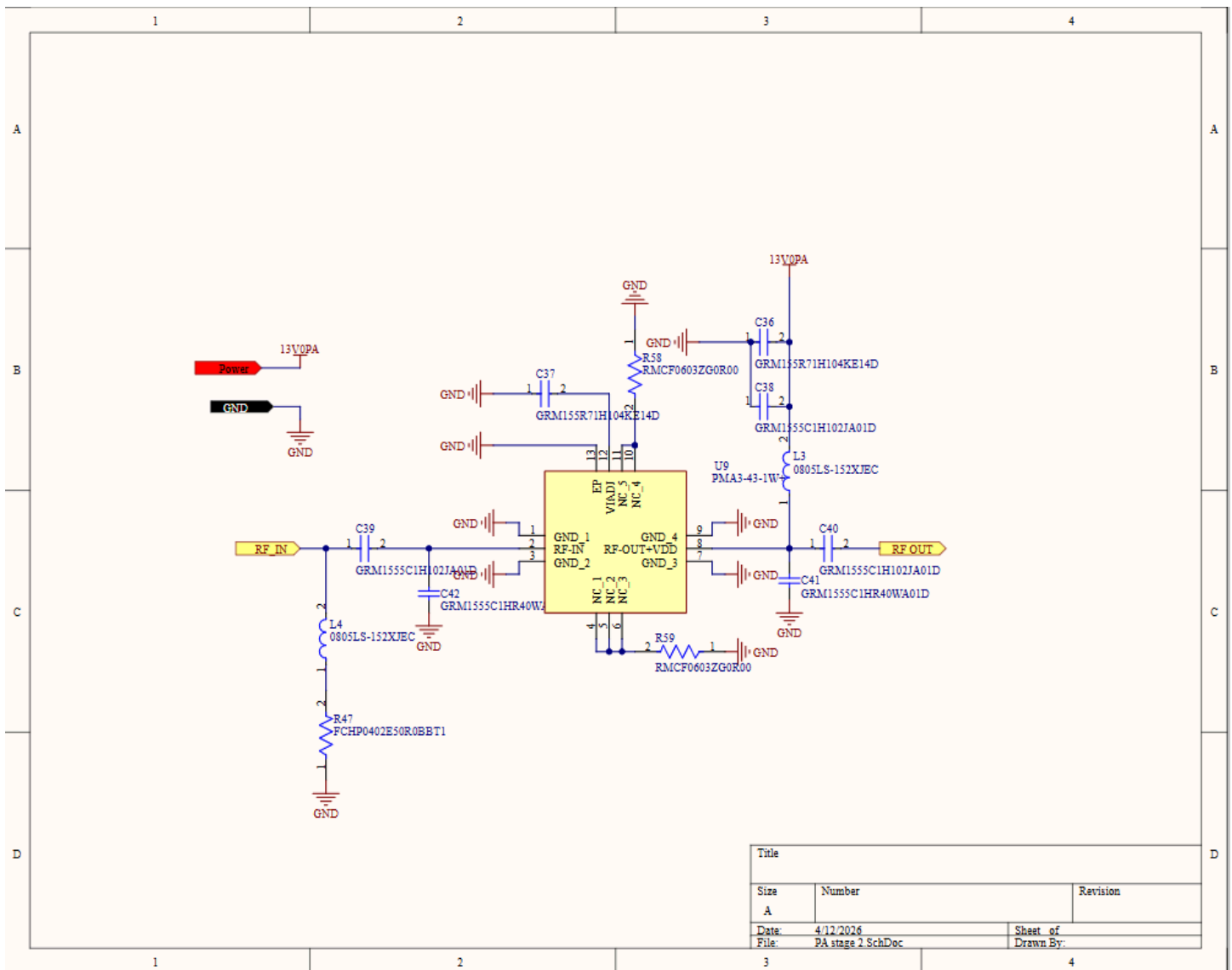
Second-stage PA sub-system schematic.
