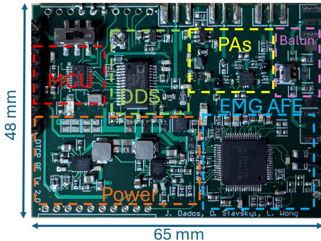
Prototype PCB with different sub-systems and dimensions.
