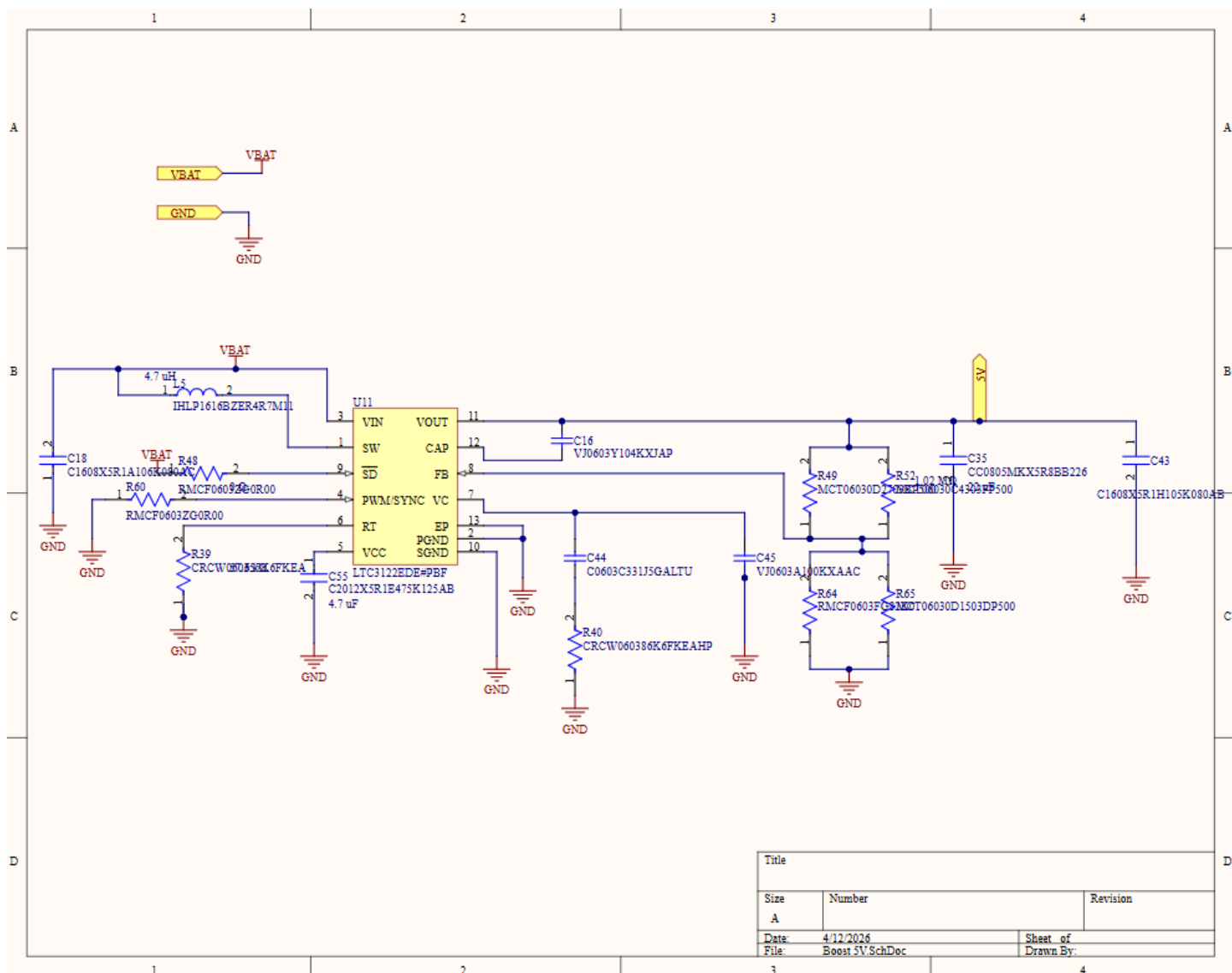
The 5V boost converter schematic.
