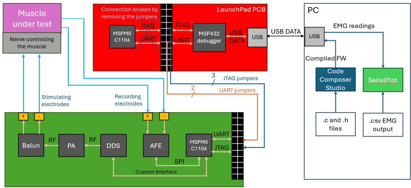
Overview of all internal and external interfaces of the device.
