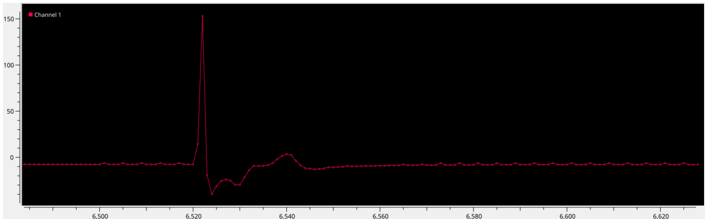
Measurement of a test EMG signal preceded by a stimulation artifact with an 8 kHz sampling rate in saline.
