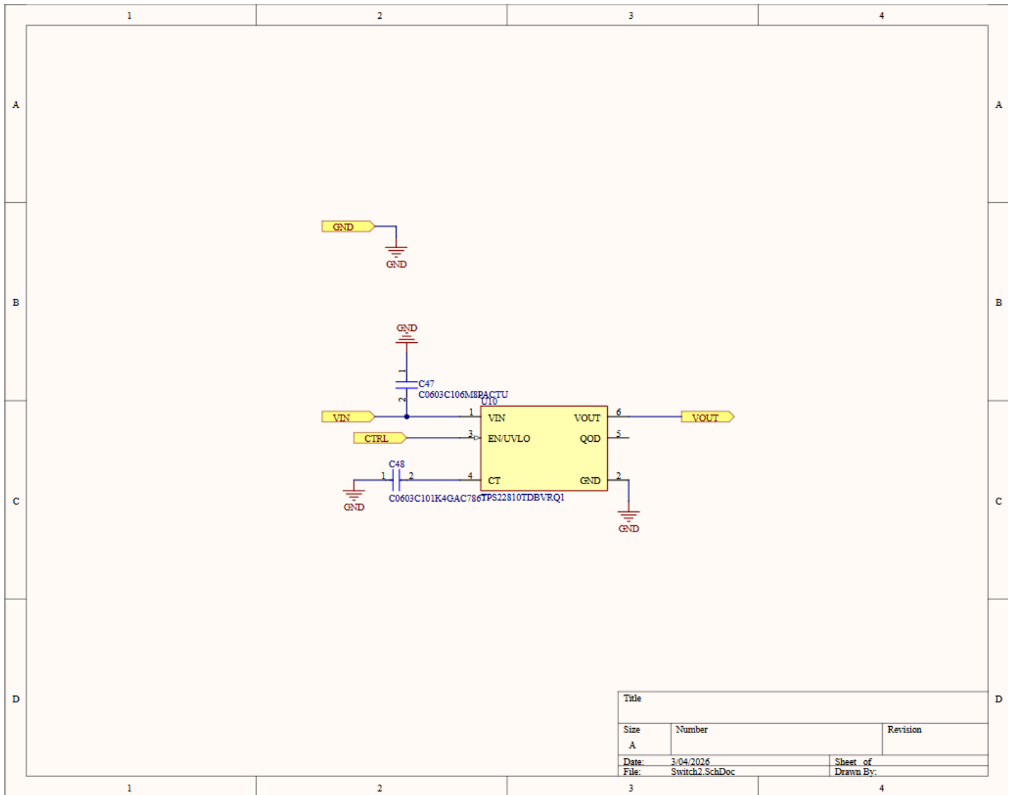
Power switch sub-system schematic
