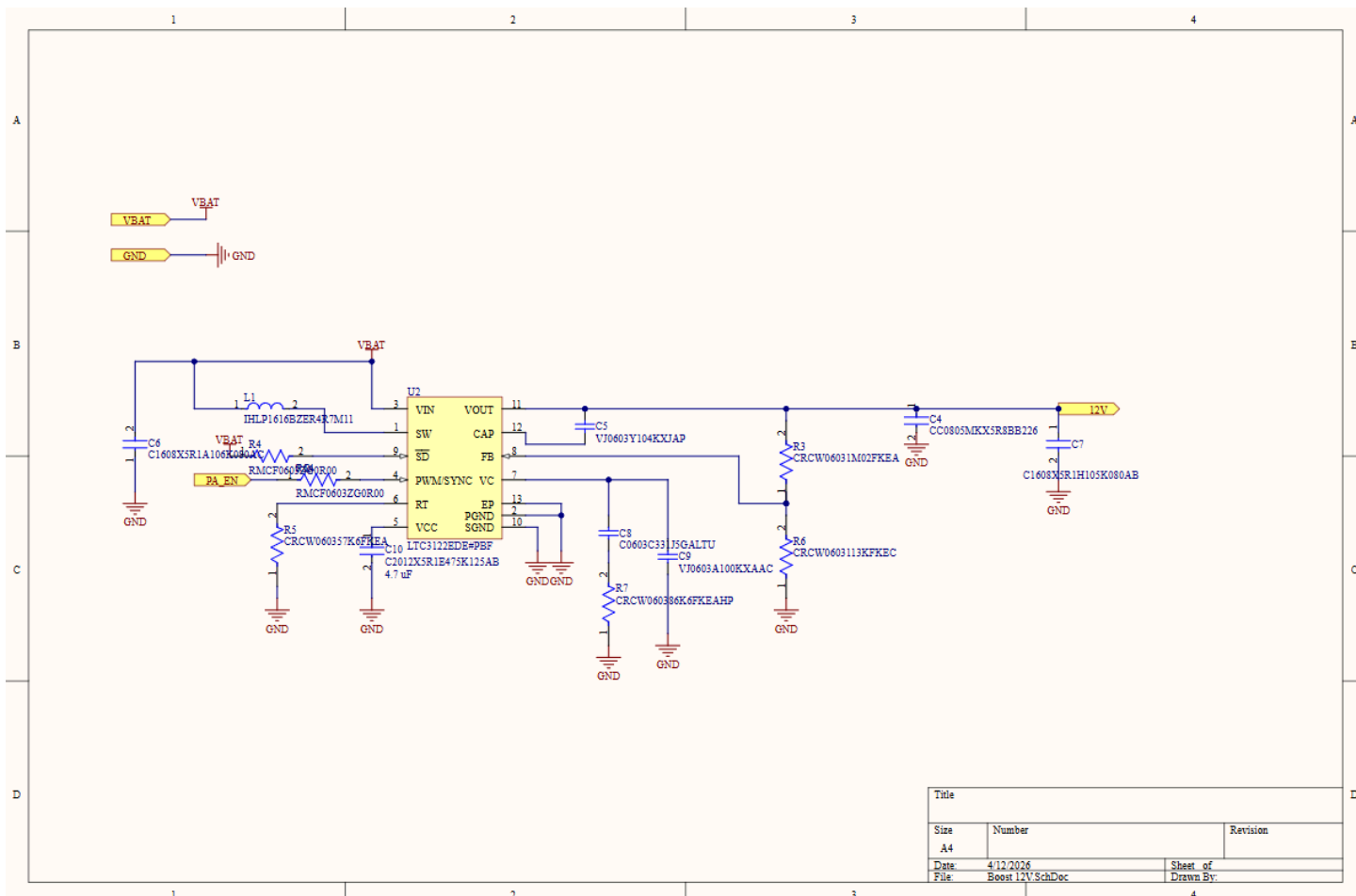
The 12V boost converter schematic.
