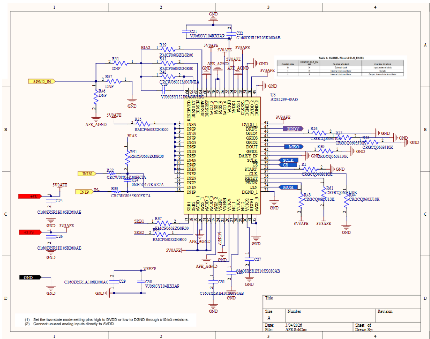
AFE sub-system schematic.
