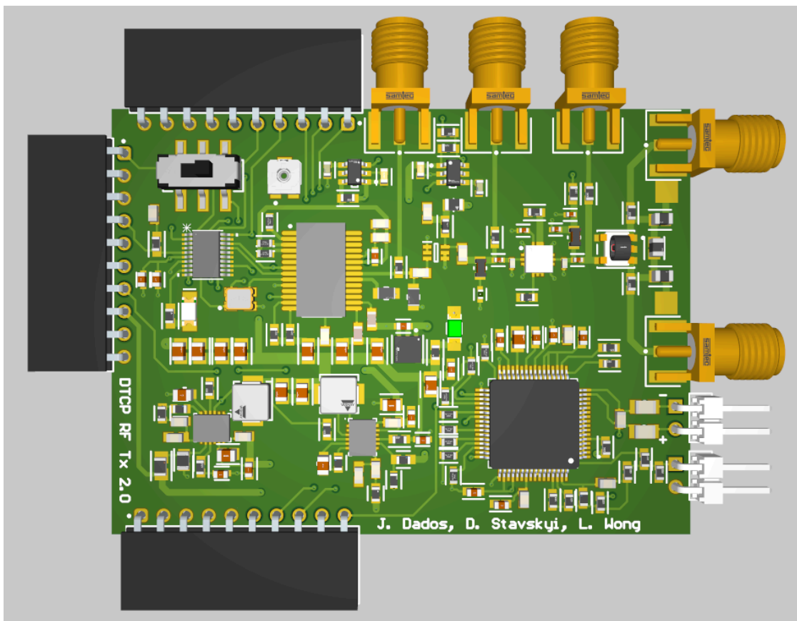
3D render of the assembled board.
