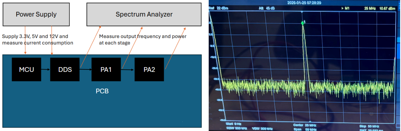
Testing methodology for the RF circuit and the final reading of output power meeting the requirement of 1W (with a 20 dB attenuator in series, bringing the signal from 30.67 dBm down to 10.67 dBm)
